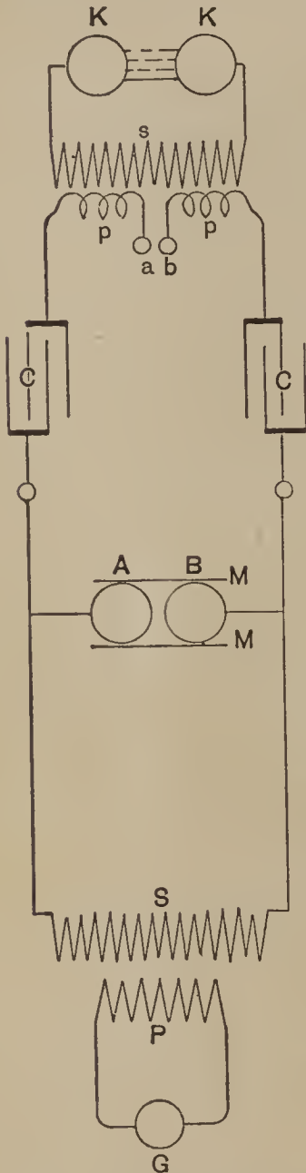
FIG. 2.—IMITATING THE SPARK OF A HOLTZ MACHINE.
