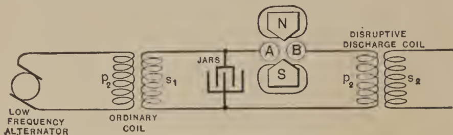
FIG. 5.—ARRANGEMENT WITH LOW-FREQUENCY ALTERNATOR AND IMPROVED DISCHARGER.
