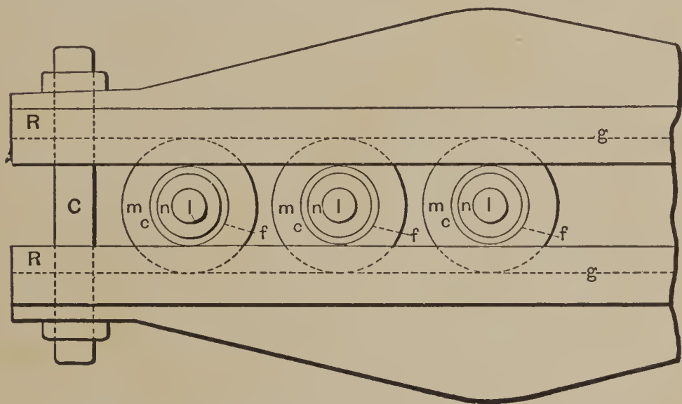
FIG. 7.—DISCHARGER WITH MULTIPLE GAPS.
