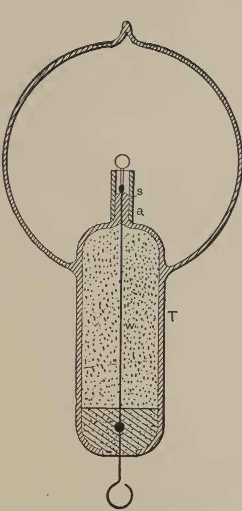
FIG. 21.—IMPROVED BULB WITH NON-CONDUCTING BUTTON.
