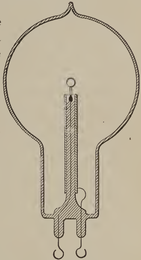
FIG. 20.—BULB FOR EXPERIMENTS WITH CONDUCTING TUBE.
