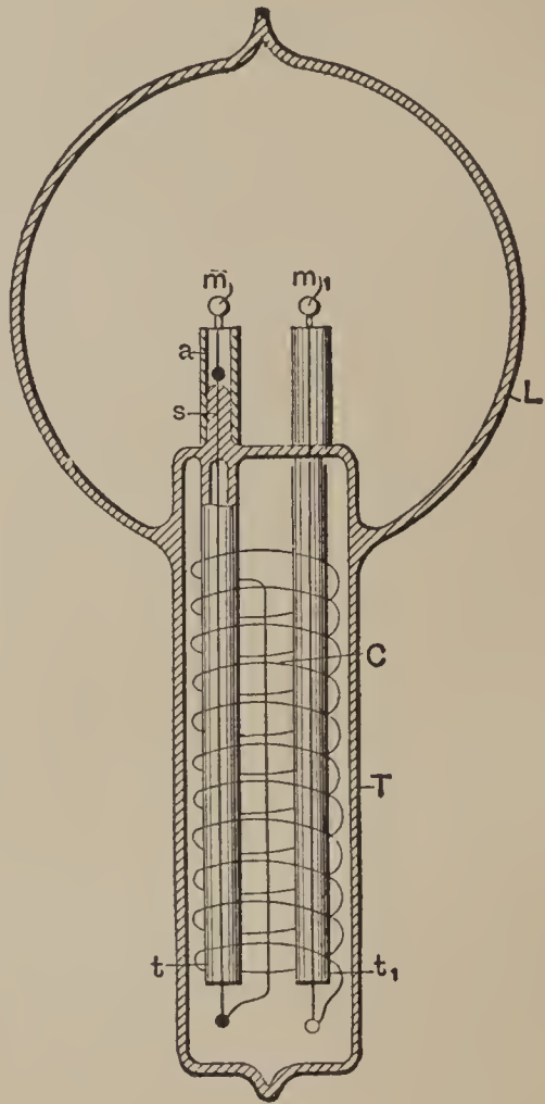
FIG. 33.—ELECTRO-DYNAMIC INDUCTION LAMP.
