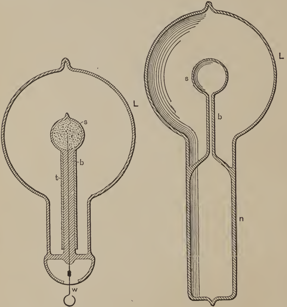
FIG. 12. BULBS FOR PRODUCING ROTATING BRUSH.
