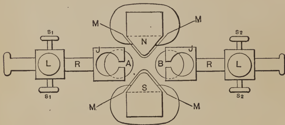
FIG. 4.—ARRANGEMENT OF IMPROVED DISCHARGER AND MAGNET.
