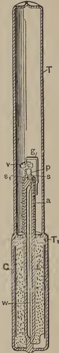
FIG. 35.—CROOKES' EXPERIMENT IN ELECTROSTATIC FIELD.
